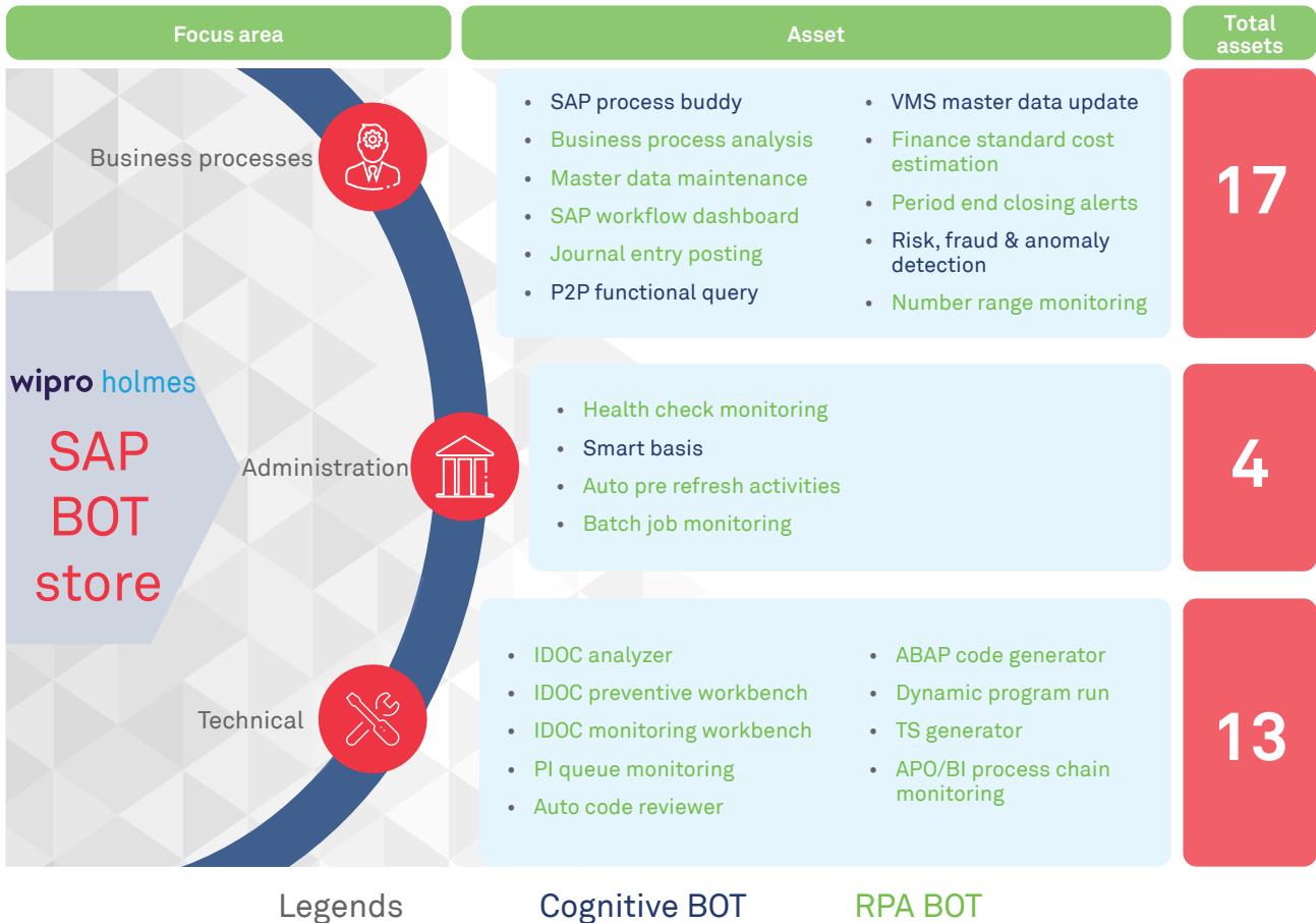
Fig. 2: SAP automation asset repository
